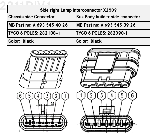
Tab17- Side Right lamp interface connector X2509
