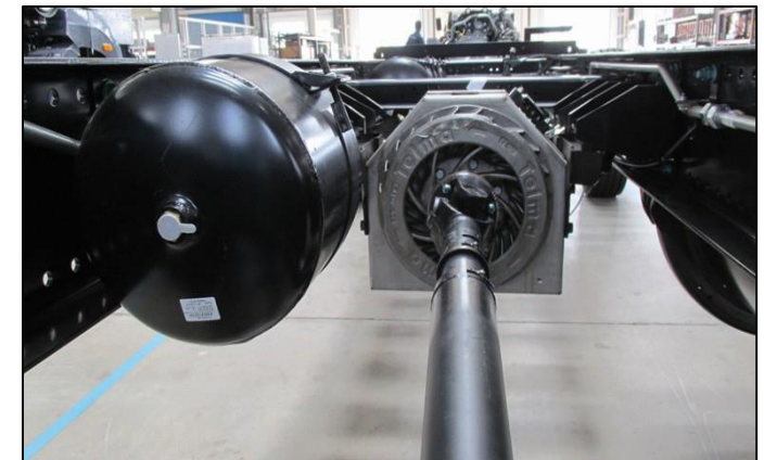
Retarder
