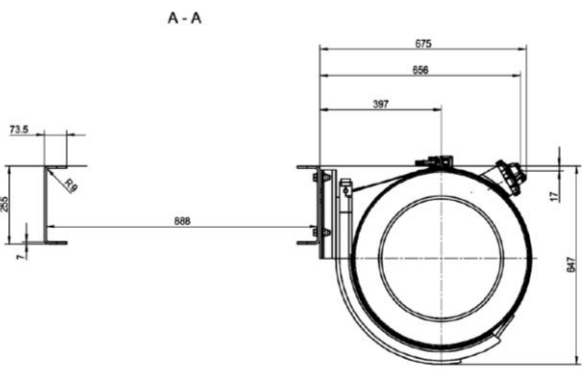
Disposition of fuel tank Capacity 390L
