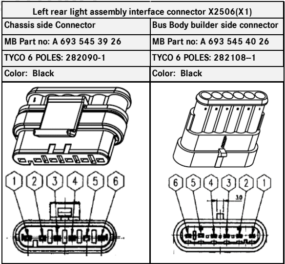
Tab18 - Left rear light assembly interface connector X2506(X1)
