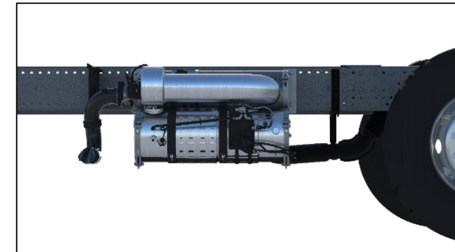
SCR system
