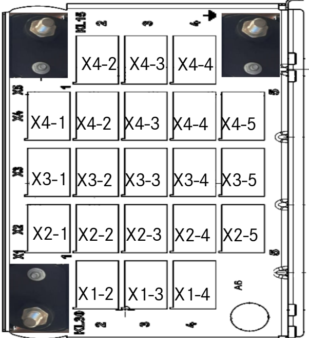
Interconnector Board connectors position
