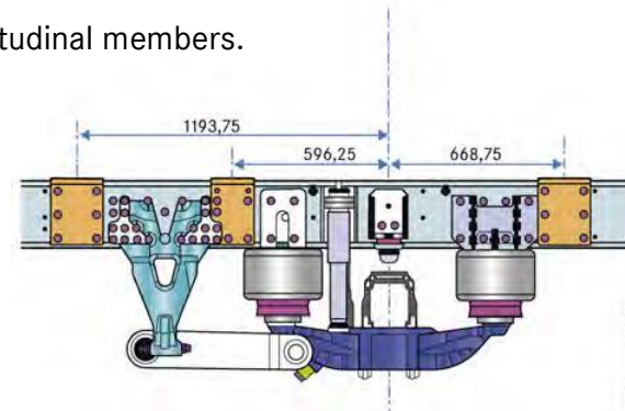
Body attachment plates-Rear
