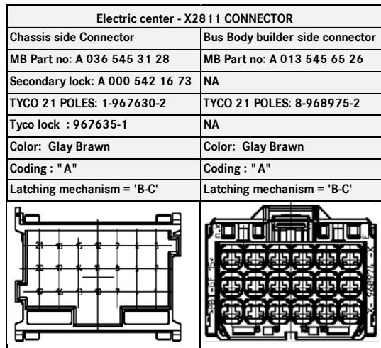
Bus Body Interconnector
