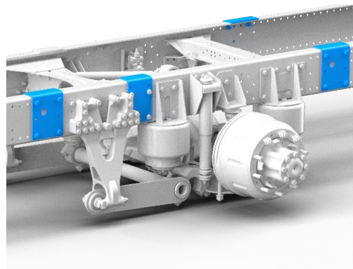
Body attachment plates at Front
