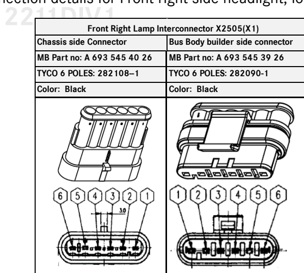
Tab14- Front Right lamp interface connector X2505(X1)
