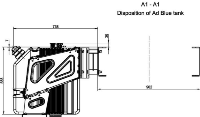
Capacity 60L
