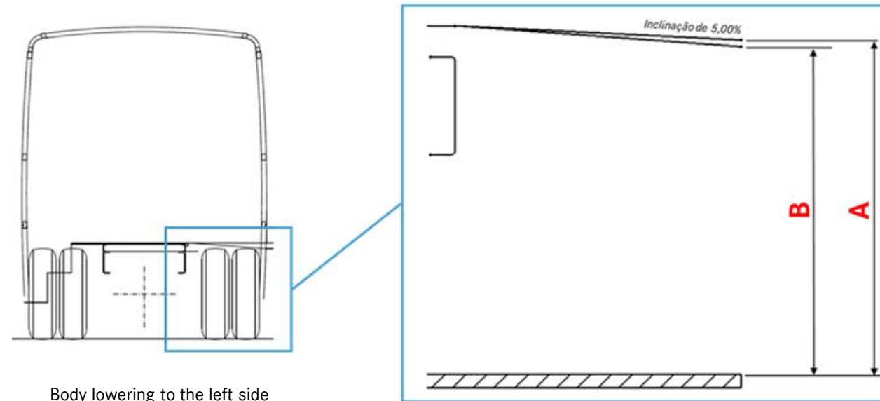
Body lowering to the left side
