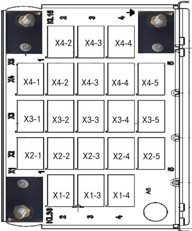
Connector switchboard
