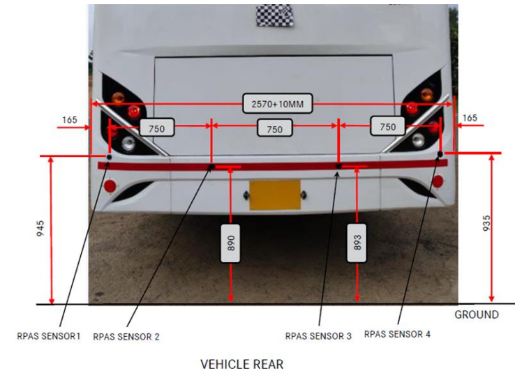
Dimension shown for reference only
